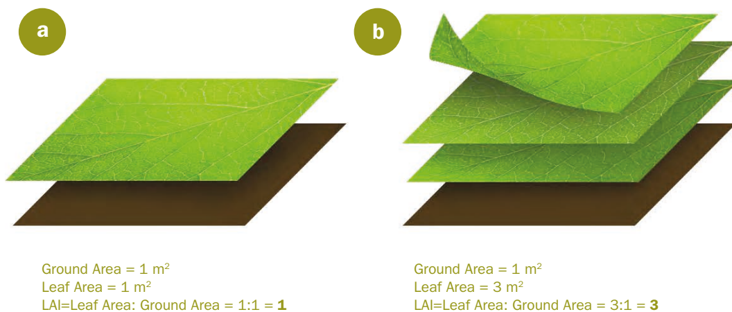
Figure I. Conceptual diagram of a plant canopy where (a) LAI = 1 or (b) LAI = 3.
